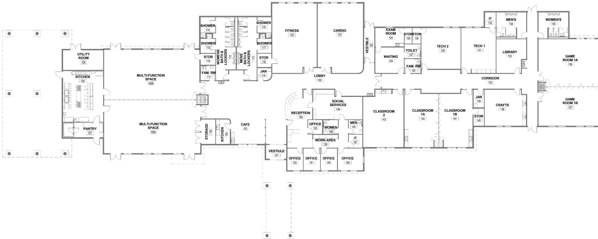
1 MAIN FLOOR PLAN 3/32" = 1'-0"
